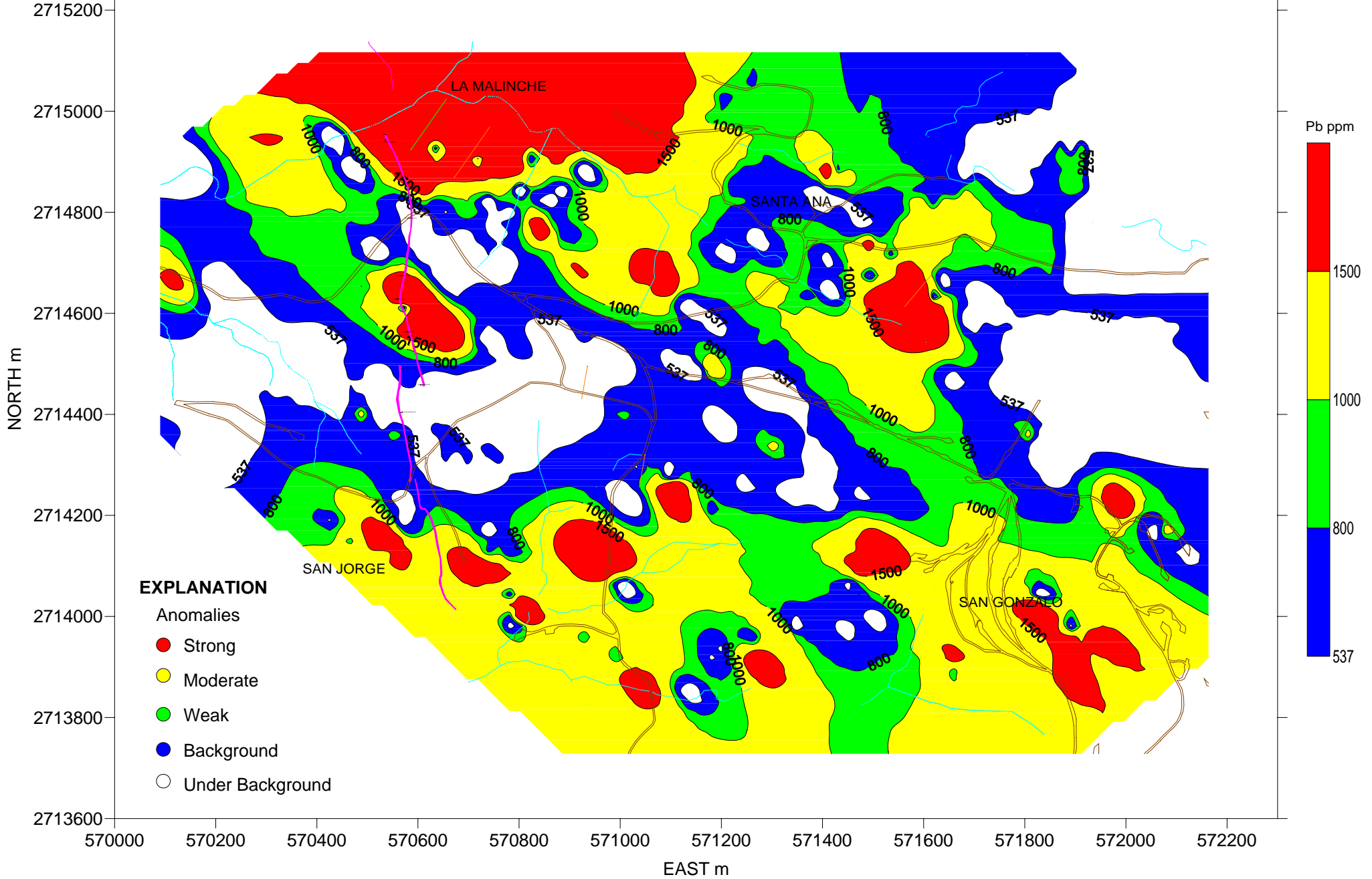
FIG. 24. MERCEDES AREA: Pb contours
